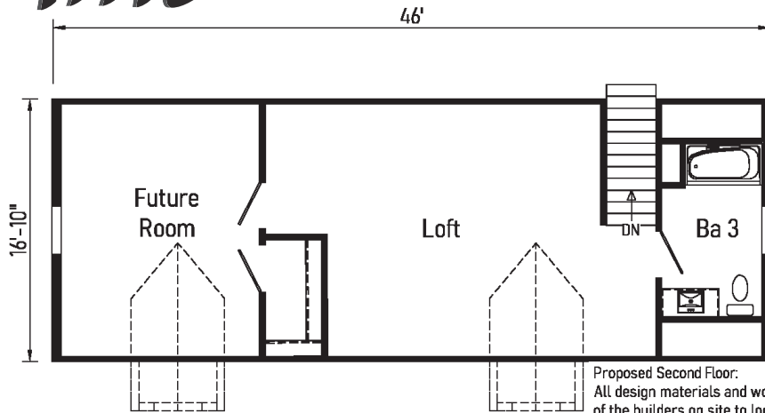
SECOND FLOOR
